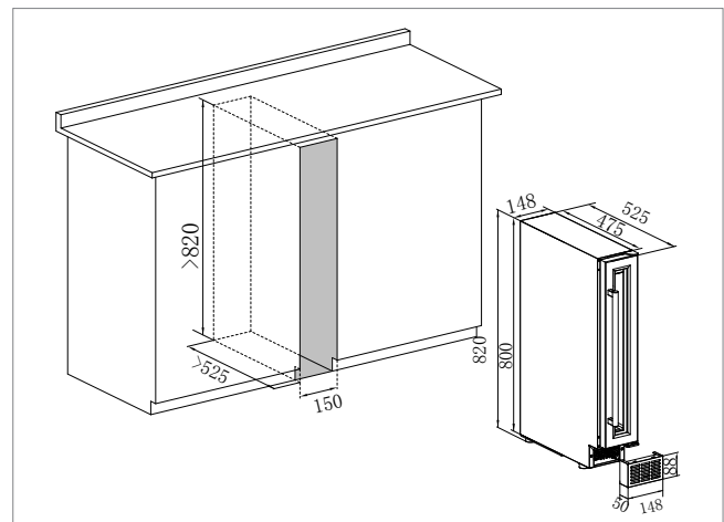
Model: OX15SRB, SOMX15SRB
