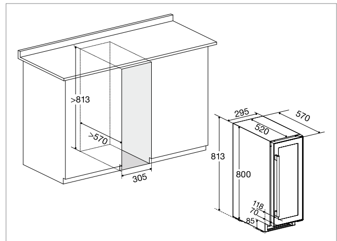
Model: OX30DX, OX30DRB, OX30DRW, SOMX30DRB, PRESX30SB, STX30DRB, STX30DS
