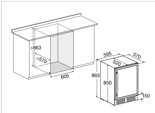
Model: WPQ60SCS, WPQ60SCB, WPQ60DCS, WPQ60DCB, WFQ60SCS, WFQ60SCB, EX60DRB, EX60DRW, EX60DX
