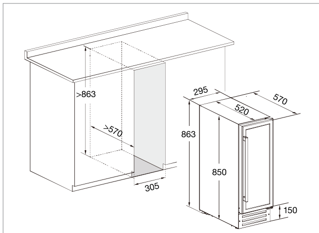
Model: WPQ30SCS, WPQ30SCB
