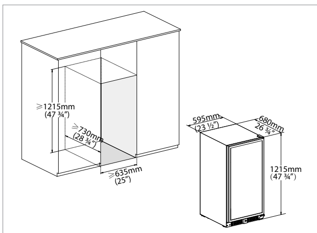
Model: WP120DCS, WP120DCB
