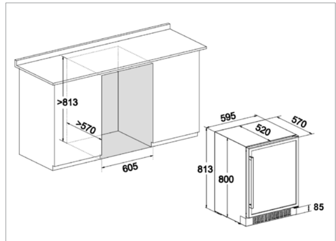
Model: WPX60DCS, WPX60DCB, OX60DRB, OX60DRW, OX60DX, CPROX60SRB, CPROX60SX, SOMX60DRB, PRESX60DB, PRESPROX60SRB, STX60DS, STX60DRB
