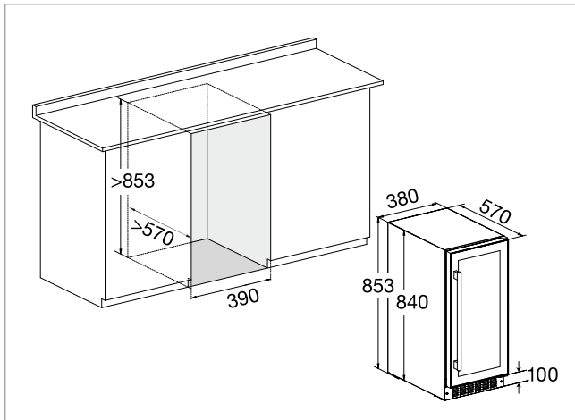
Model: WPQ38SCS, WPQ38SCB, WPQ38DCS, WPQ38DCB, SOMQ38DRB, PRESQ38DB
