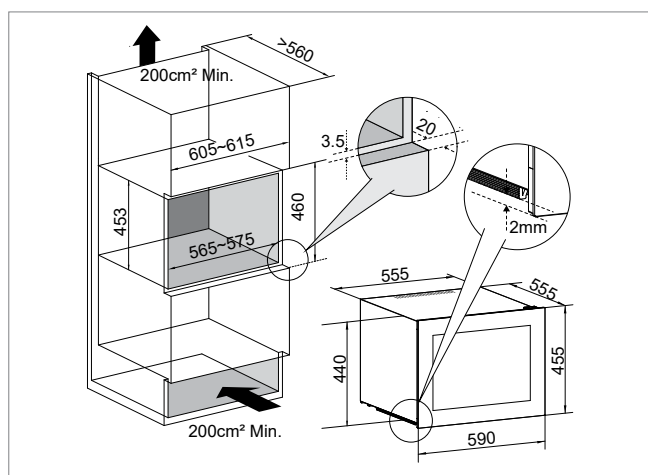
Model: OZ45SX, OZ45SB, OZ45SW
