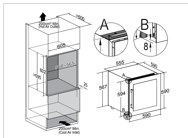
Model: OZ60SB, OZ60DB, OZ60DX, OZ60DW, STZ60SB, STZ60SX
